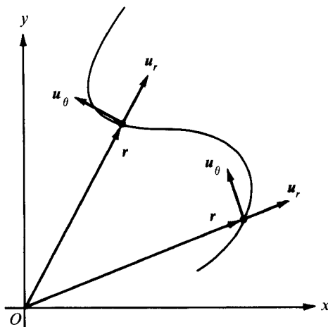
FIGURE 14.16 The unit vectors \mathbf{u}_r and \mathbf{u}_\theta .
