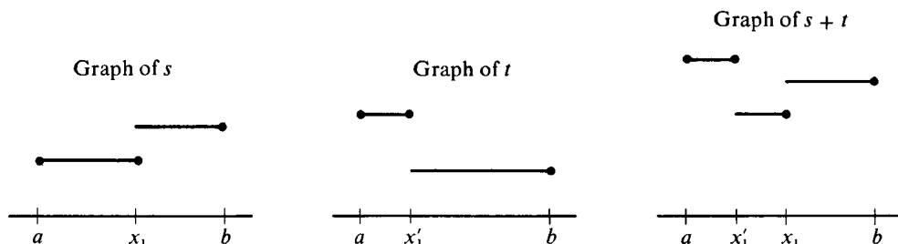
FIGURE 1.21 The sum of two step functions.
