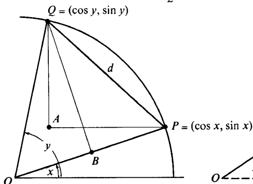
FIGURE 2.8 Geometric proof of the formula for \cos(y-x) .
